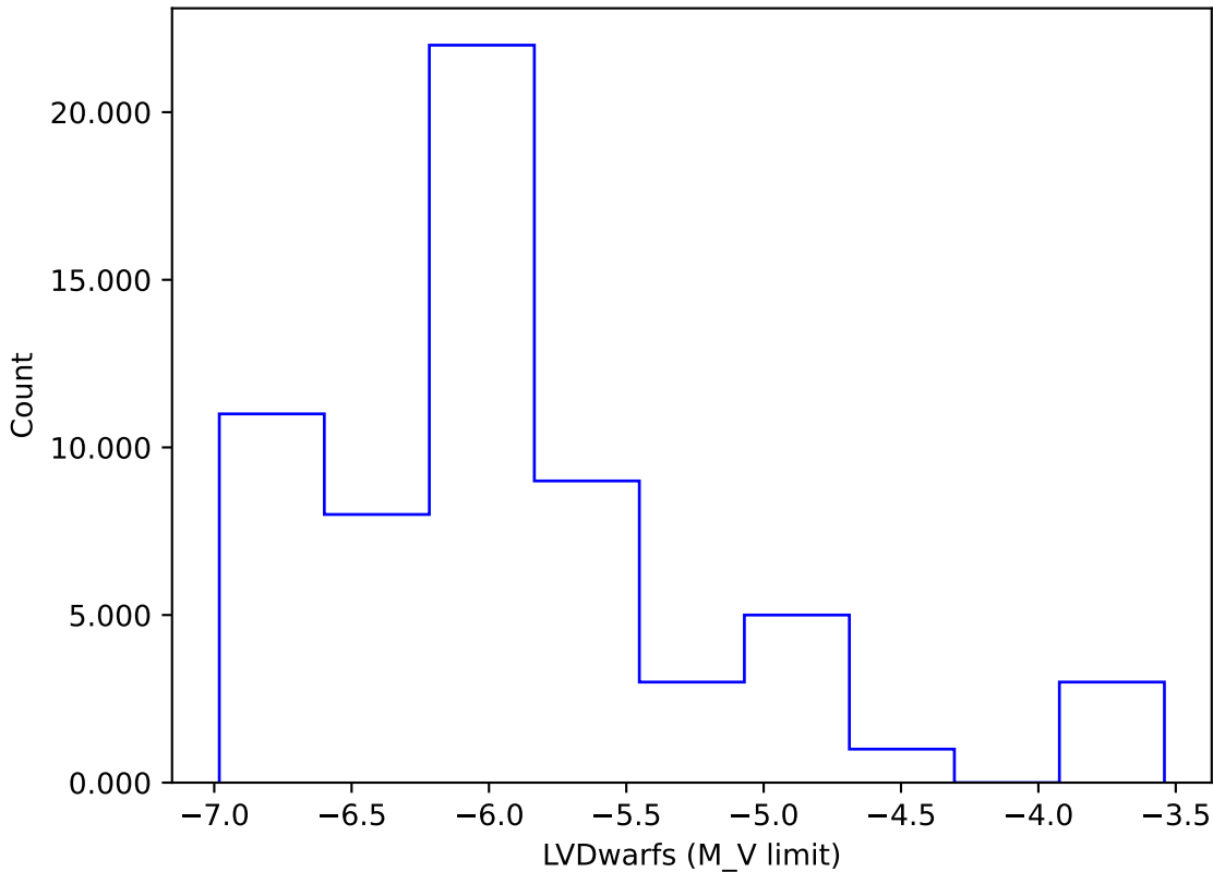
ddf_acor_sf15_lsf40_lsr10_v3.4_10yrs gi: LVDwarfs
