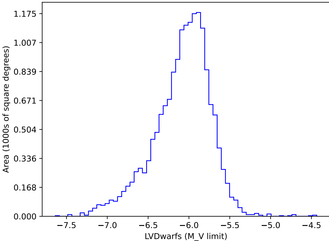
ddf_acor_sf15_lsf40_lsr10_v3.4_10yrs gi: LVDwarfs
