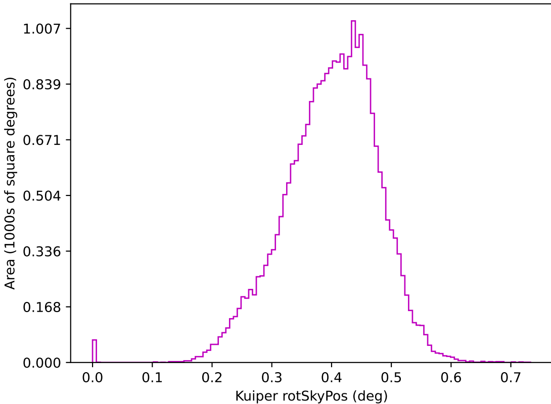
ddf_acor_sf15_lsf40_lsr10_v3.4_10yrs z: Kuiper rotSkyPos
