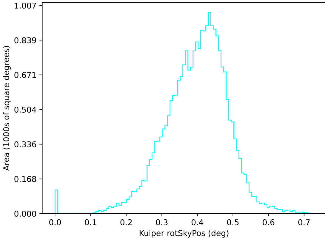
ddf_acor_sf15_lsf40_lsr10_v3.4_10yrs u: Kuiper rotSkyPos
