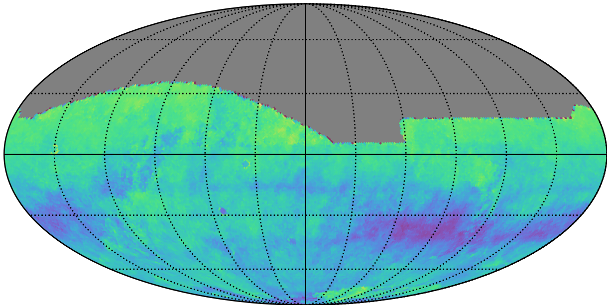
ddf_acor_sf15_lsf40_lsr10_v3.4_10yrs r: Kuiper rotSkyPos
