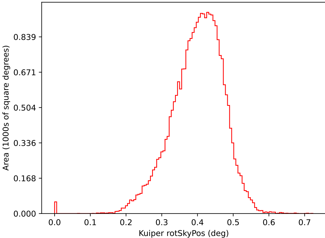
ddf_acor_sf15_ls40_lsr10_v3.4_10yrs i: Kuiper rotSkyPos
