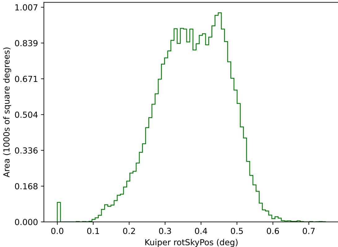
ddf_acor_sf15_lsf40_lsr10_v3.4_10yrs g: Kuiper rotSkyPos
