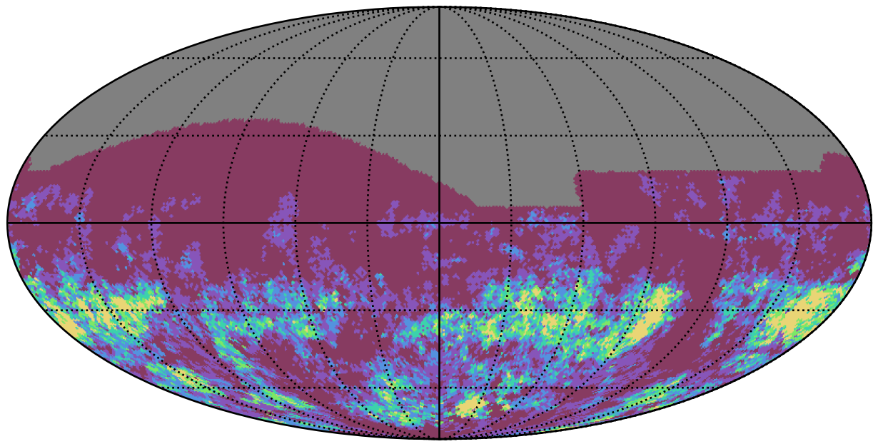
ddf_acor_sf15_lsf40_lsr10_v3.4_10yrs r band: Gaps_7hr
