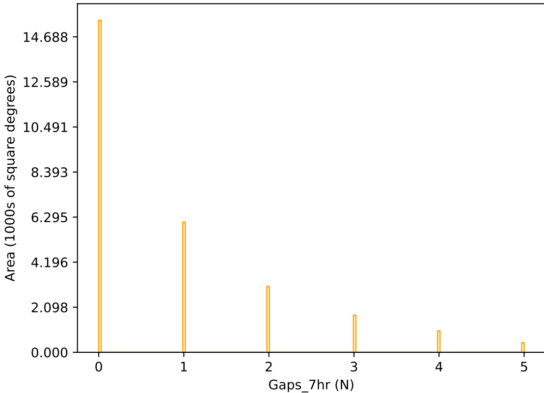
ddf_acor_sf15_lsf40_lsr10_v3.4_10yrs r band: Gaps_7hr
