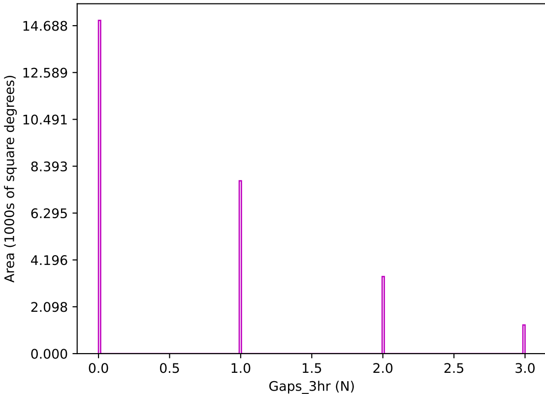
ddf_acor_sf15_lsf40_lsr10_v3.4_10yrs z band: Gaps_3hr
