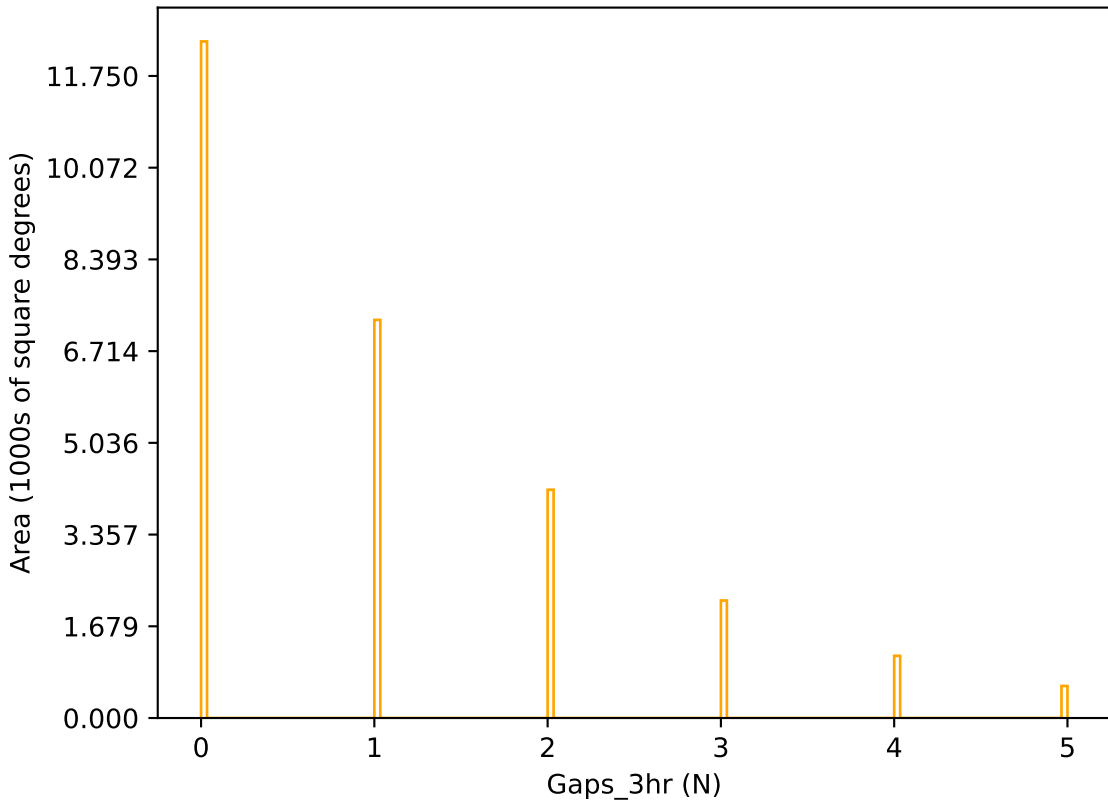
ddf_acor_sf15_lsf40_lsr10_v3.4_10yrs r band: Gaps_3hr
