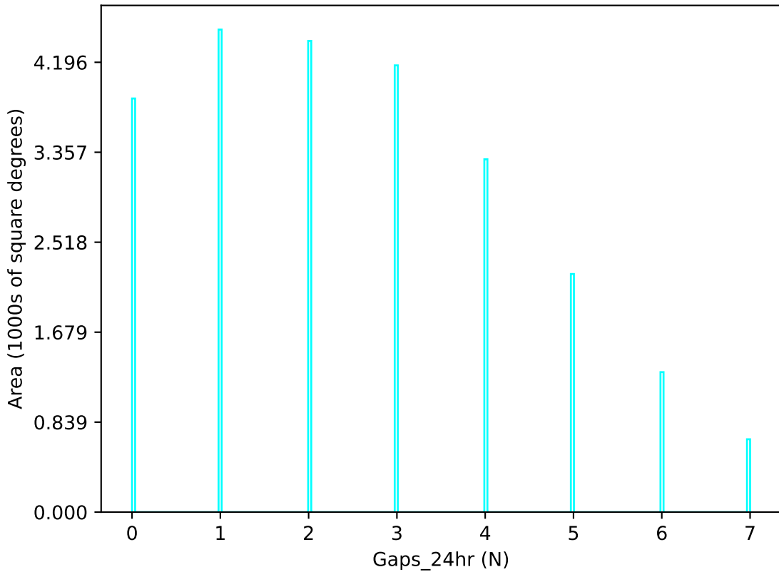
ddf_acor_sf15_lsf40_lsr10_v3.4_10yrs u band: Gaps_24hr
