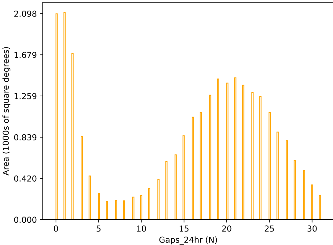
ddf_acor_sf15_ls40_lsr10_v3.4_10yrs r band: Gaps_24hr
