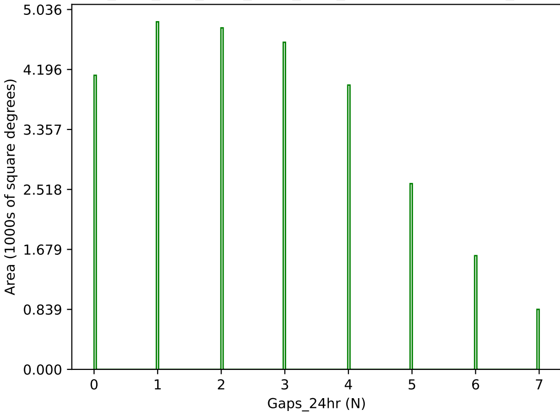
ddf_acor_sf15_lsf40_lsr10_v3.4_10yrs g band: Gaps_24hr
