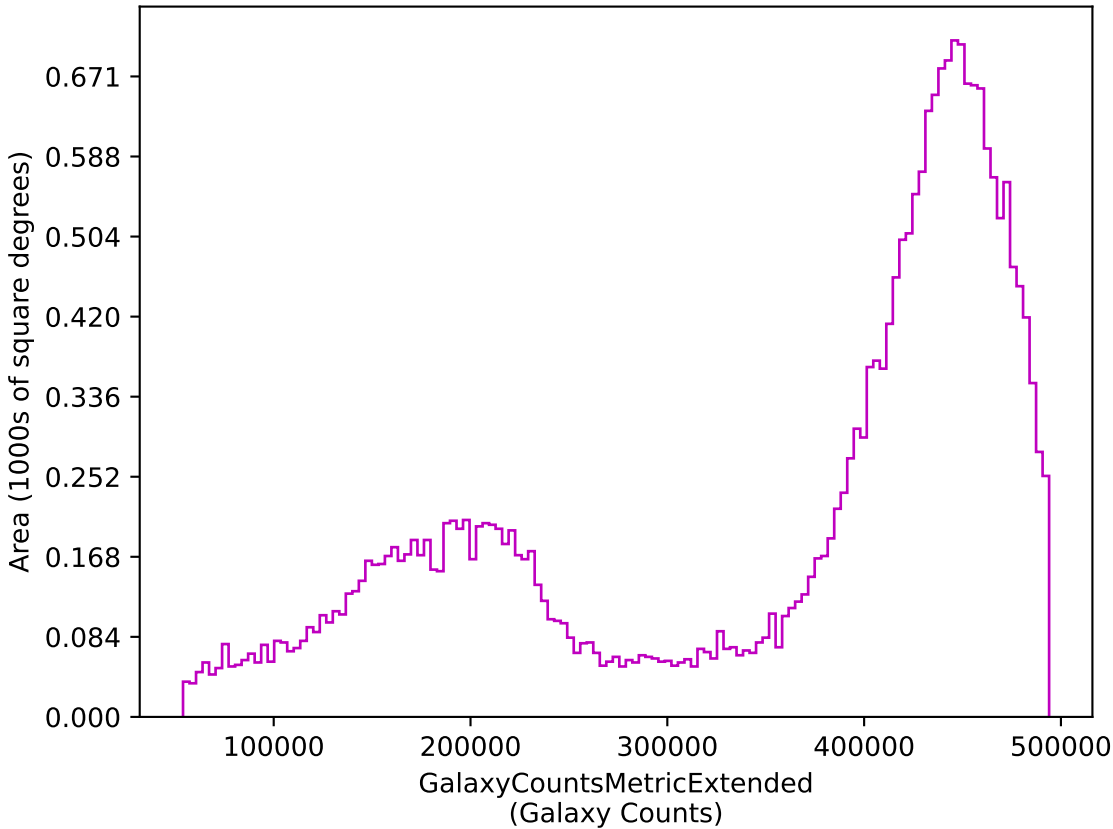
ddf_acor_sf15_lsf40_lsr10_v3.4_10yrs z: GalaxyCountsMetricExtended
