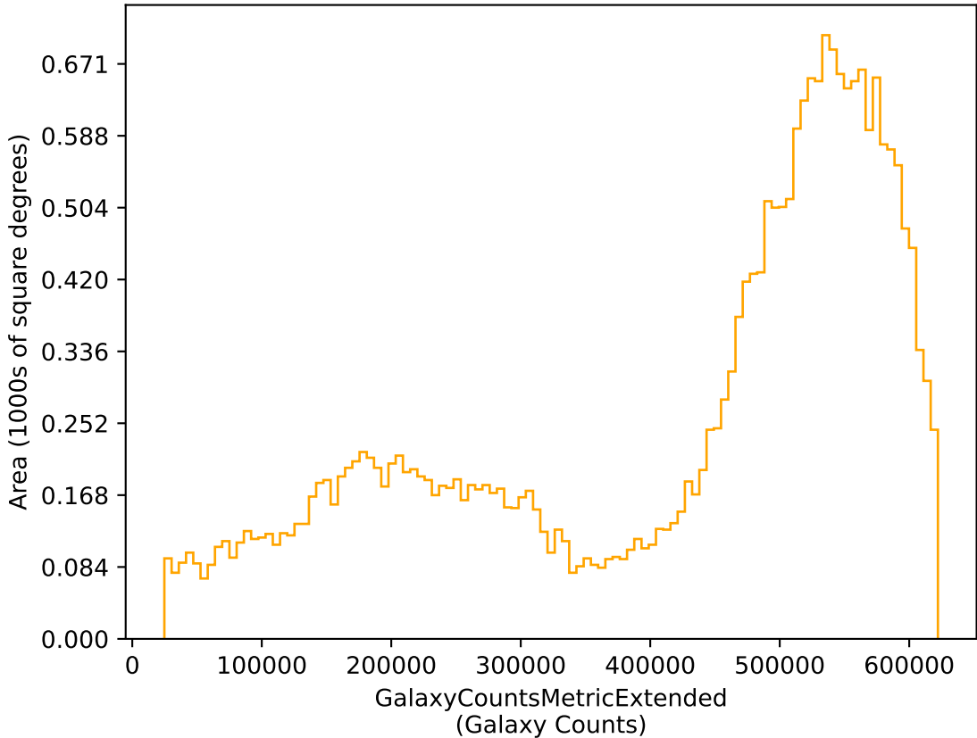
ddf_acor_sf15_lsf40_lsr10_v3.4_10yrs r: GalaxyCountsMetricExtended
