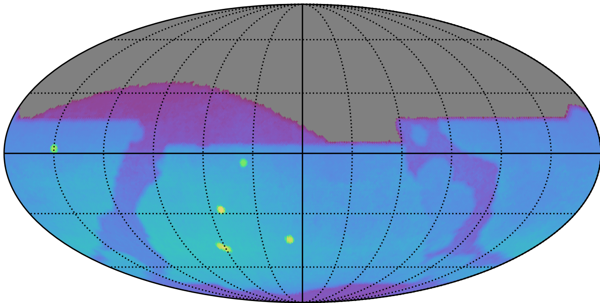
ddf_acor_sf15_lsf40_lsr10_v3.4_10yrs : Brown Dwarf, L7
