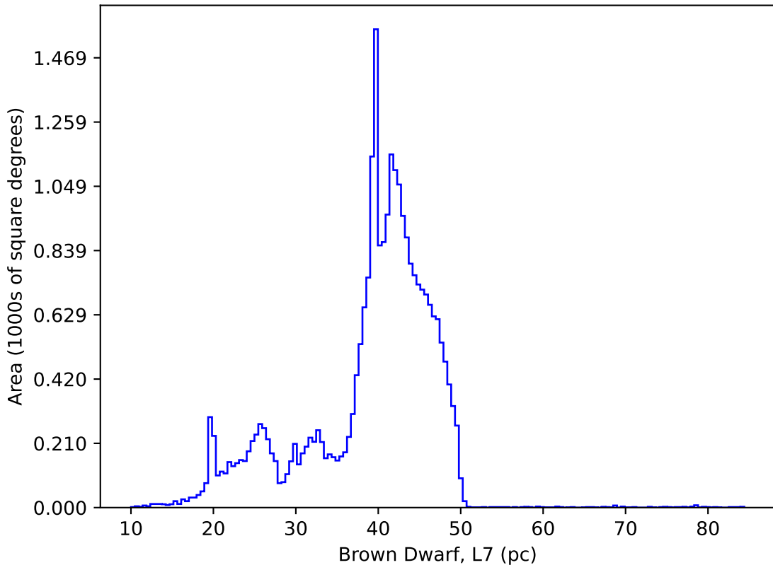
ddf_acor_sf15_lsf40_lsr10_v3.4_10yrs : Brown Dwarf, L7
