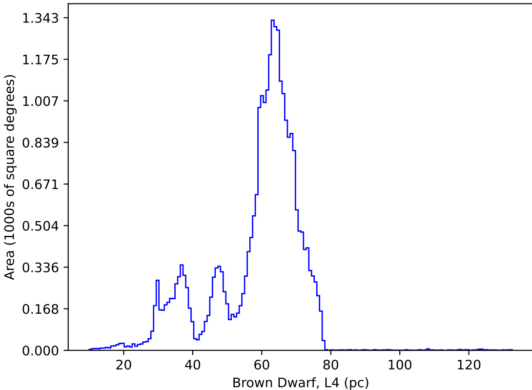
ddf_acor_sf15_lsf40_lsr10_v3.4_10yrs : Brown Dwarf, L4
