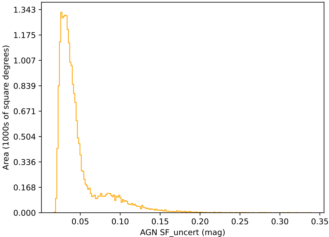
ddf_acor_sf15_lsf40_lsr10_v3.4_10yrs r band: AGN SF_uncert
