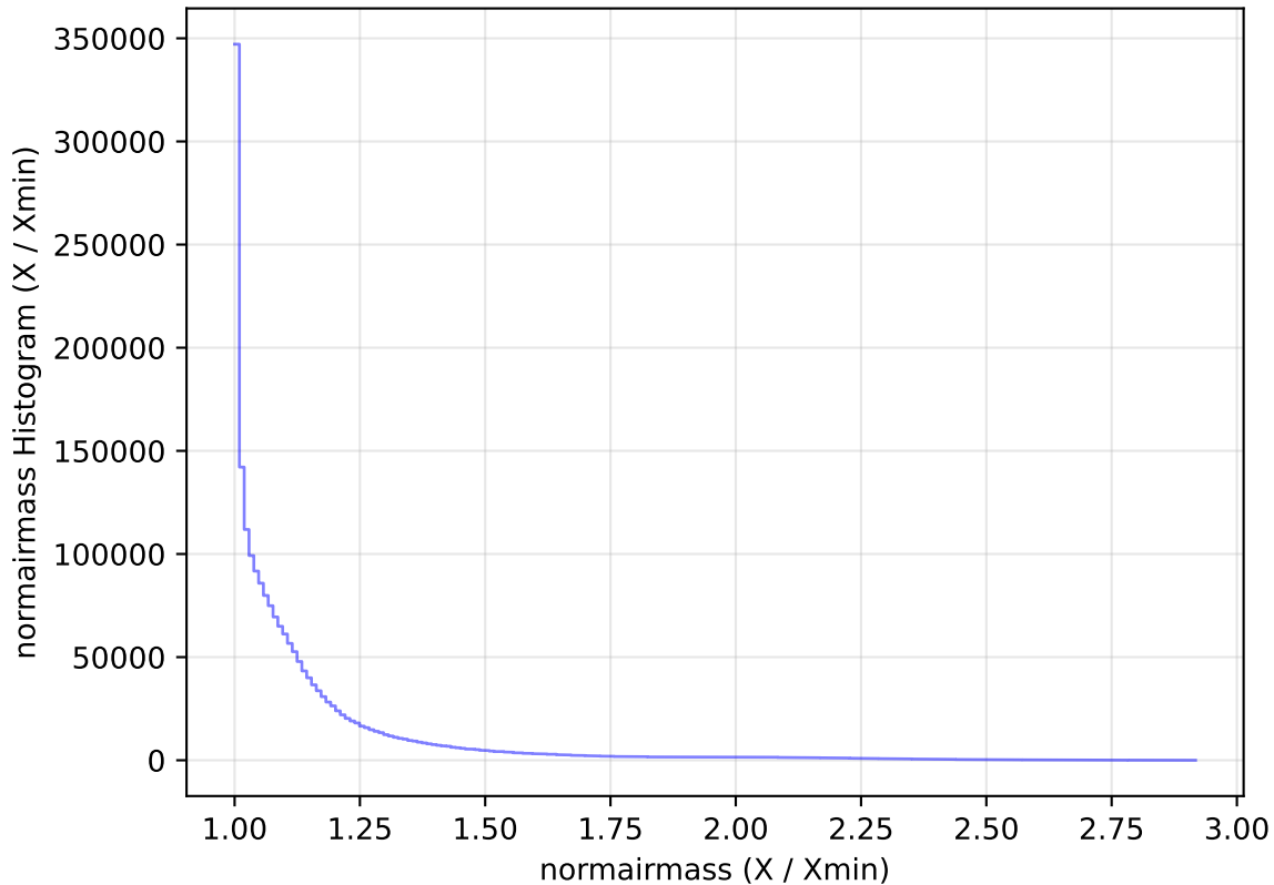
ddf_acor_sf15_lsf40_lsr10_v3.4_10yrs WFD all bands: normairmass Histogram
