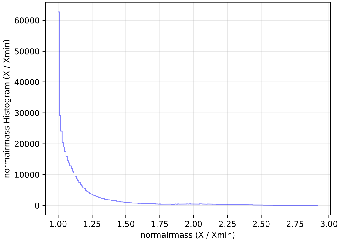
ddf_acor_sf15_lsf40_lsr10_v3.4_10yrs All sky z band: normairmass Histogram
