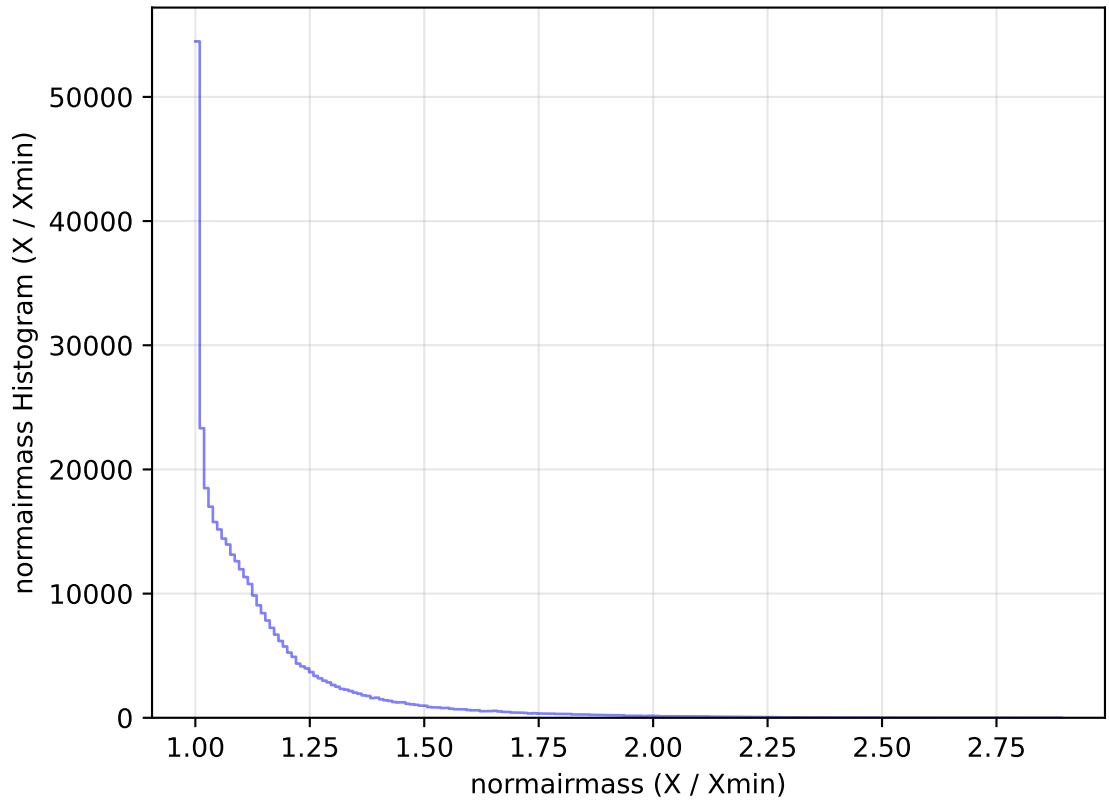
ddf_acor_sf15_lsf40_lsr10_v3.4_10yrs All sky y band: normairmass Histogram
