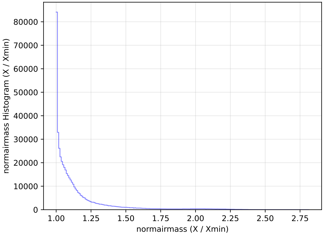
ddf_acor_sf15_lsf40_lsr10_v3.4_10yrs All sky r band: normairmass Histogram
