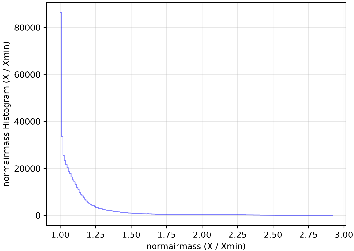
ddf_acor_sf15_lsf40_lsr10_v3.4_10yrs All sky i band: normairmass Histogram
