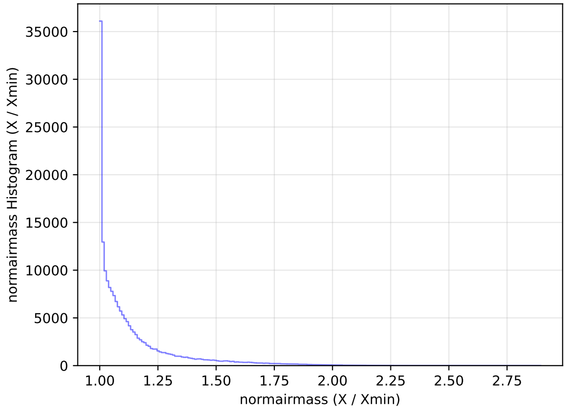
ddf_acor_sf15_lsf40_lsr10_v3.4_10yrs All sky g band: normairmass Histogram
