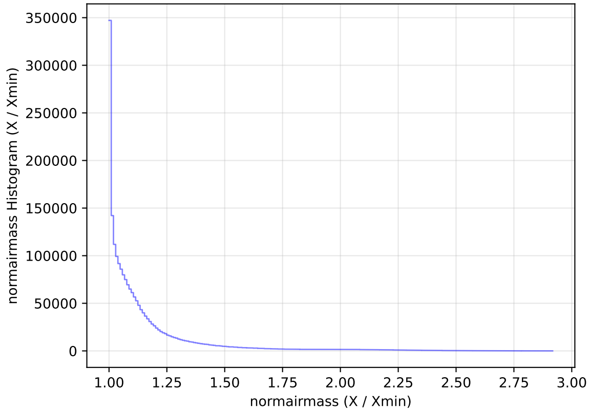
ddf_acor_sf15_lsf40_lsr10_v3.4_10yrs All sky all bands: normairmass Histogram
