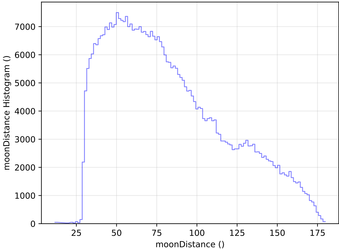
ddf_acor_sf15_Isf40_Isr10_v3.4_10yrs WFD z band: moonDistance Histogram
