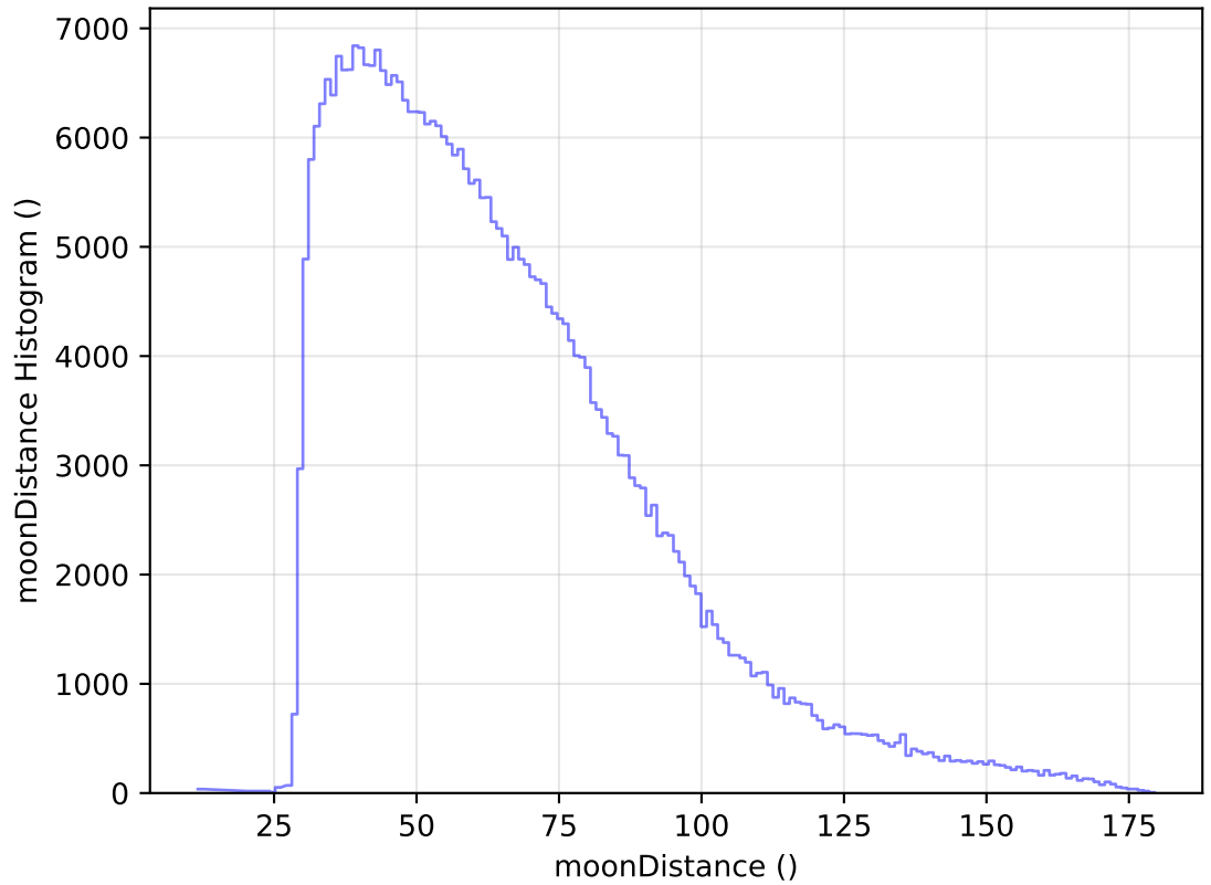
ddf_acor_sf15_lsf40_lsr10_v3.4_10yrs WFD y band: moonDistance Histogram
