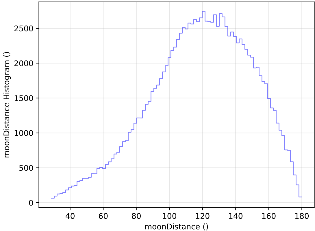
ddf_acor_sf15_lsf40_lsr10_v3.4_10yrs WFD u band: moonDistance Histogram
