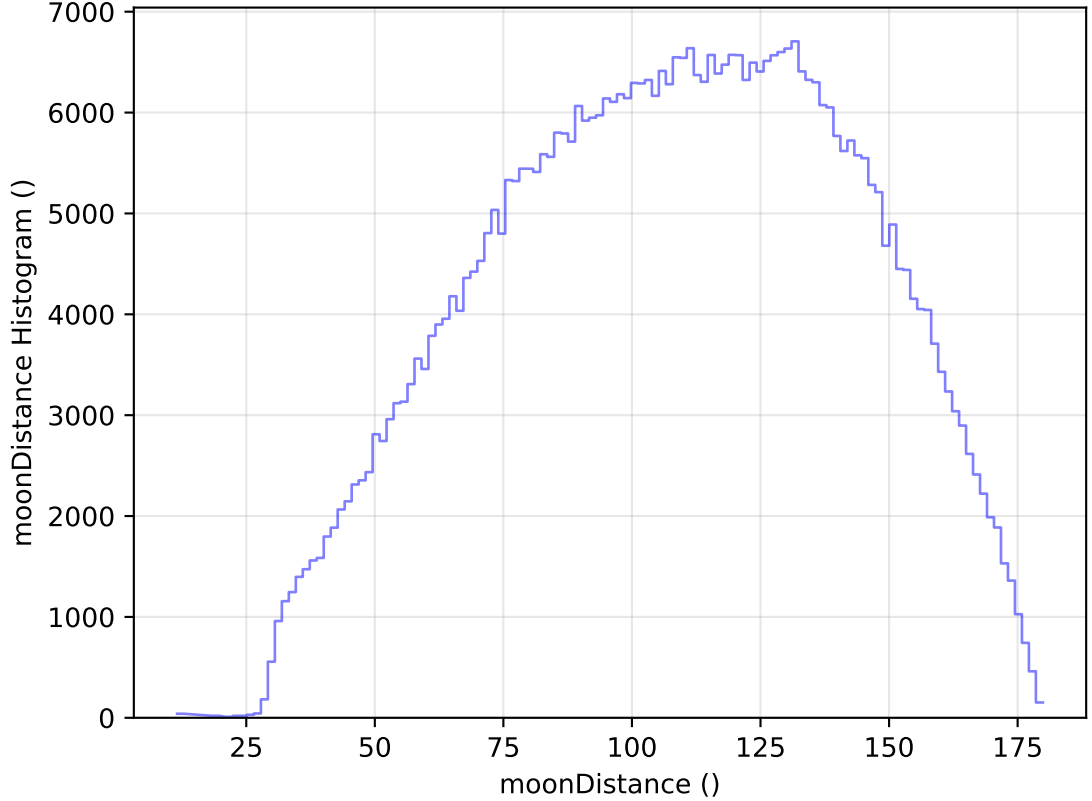
ddf_acor_sf15_lsf40_lsr10_v3.4_10yrs WFD r band: moonDistance Histogram
