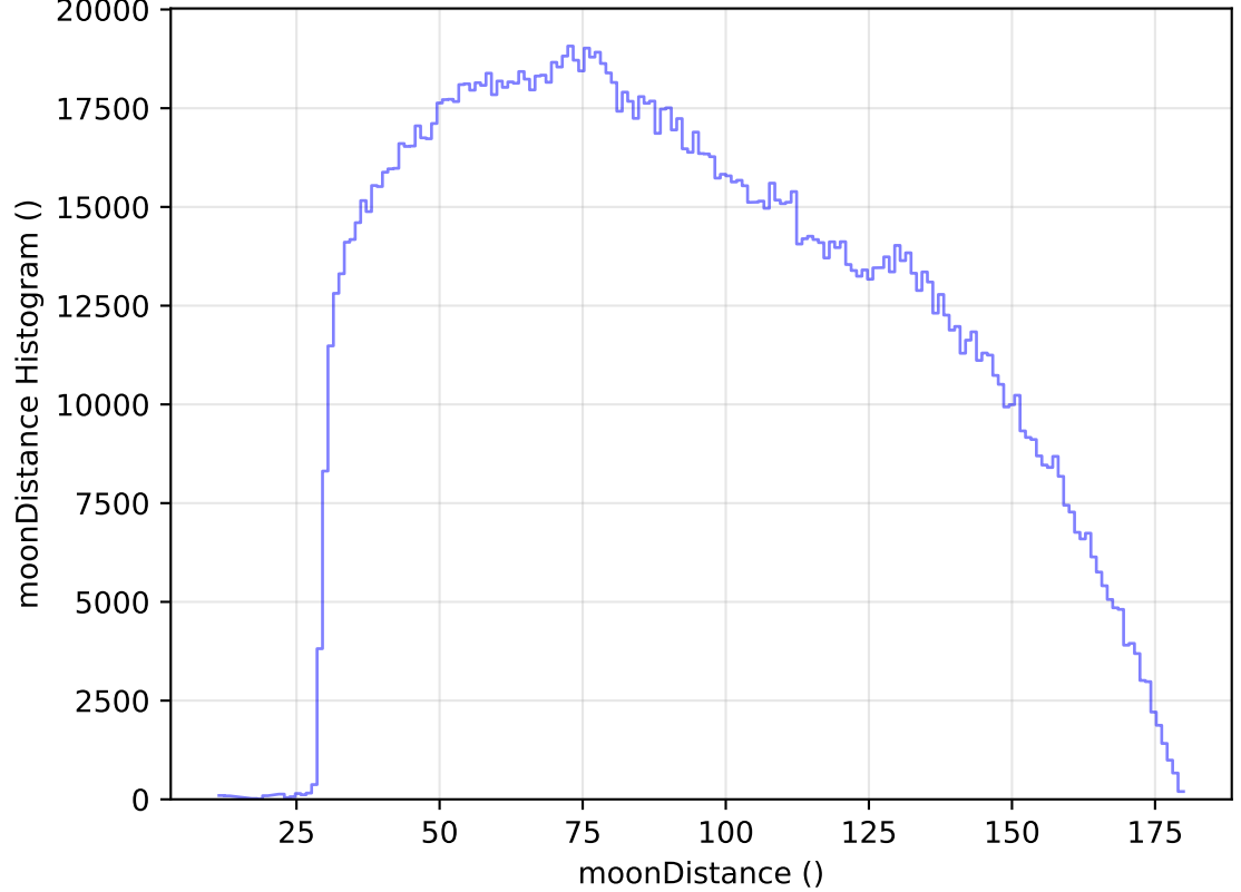
ddf_acor_sf15_lsf40_lsr10_v3.4_10yrs WFD all bands: moonDistance Histogram
