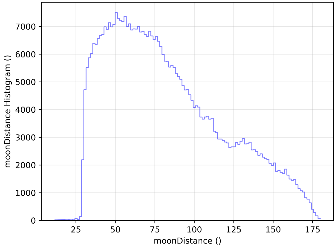
ddf_acor_sf15_lsf40_lsr10_v3.4_10yrs All sky z band: moonDistance Histogram
