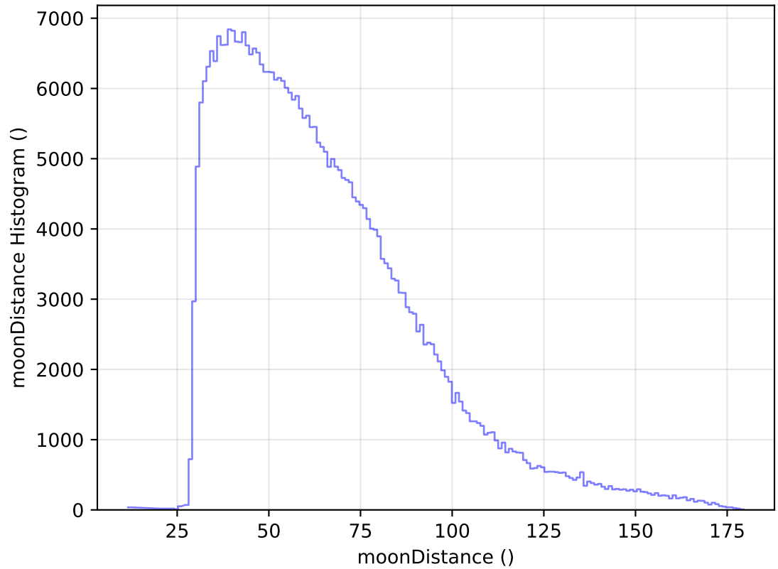
ddf_acor_sf15_lsf40_lsr10_v3.4_10yrs All sky y band: moonDistance Histogram
