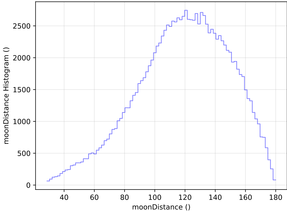
ddf_acor_sf15_lsf40_lsr10_v3.4_10yrs All sky u band: moonDistance Histogram
