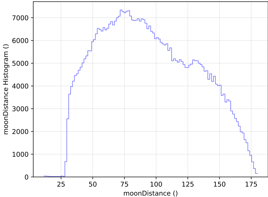
ddf_acor_sf15_lsf40_lsr10_v3.4_10yrs All sky i band: moonDistance Histogram
