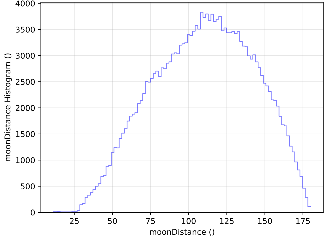
ddf_acor_sf15_lsf40_lsr10_v3.4_10yrs All sky g band: moonDistance Histogram
