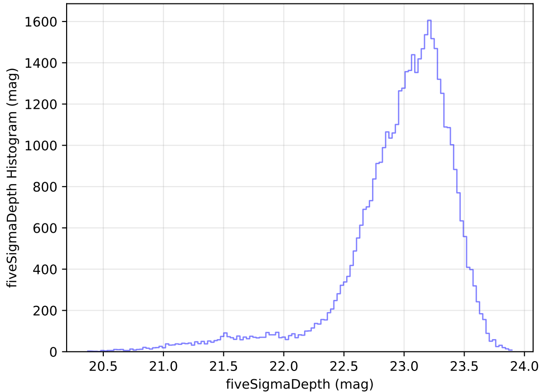
ddf_acor_sf15_lsf40_lsr10_v3.4_10yrs Yr 1 z band: fiveSigmaDepth Histogram
