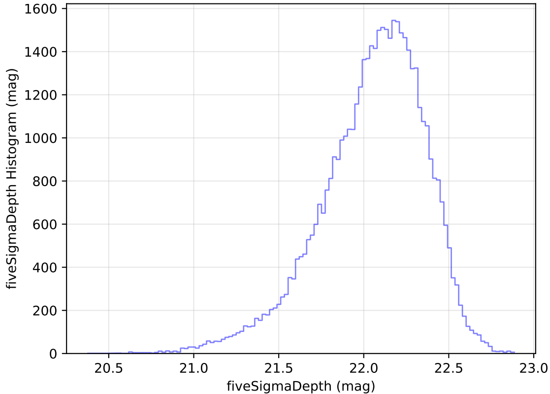
ddf_acor_sf15_lsf40_lsr10_v3.4_10yrs Yr 1 y band: fiveSigmaDepth Histogram
