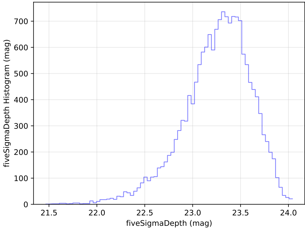
ddf_acor_sf15_lsf40_lsr10_v3.4_10yrs Yr 1 u band: fiveSigmaDepth Histogram
