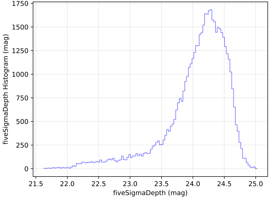
ddf_acor_sf15_lsf40_lsr10_v3.4_10yrs Yr 1 r band: fiveSigmaDepth Histogram
