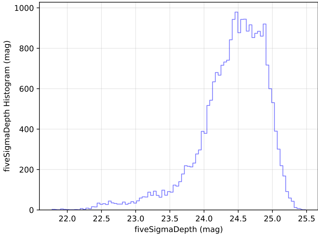
ddf_acor_sf15_lsf40_lsr10_v3.4_10yrs Yr 1 g band: fiveSigmaDepth Histogram
