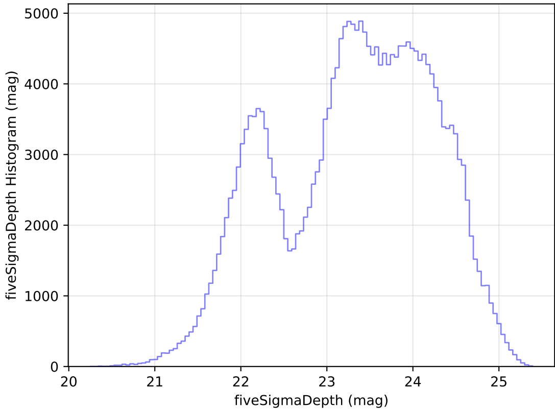
ddf_acor_sf15_lsf40_lsr10_v3.4_10yrs Yr 1 all bands: fiveSigmaDepth Histogram
