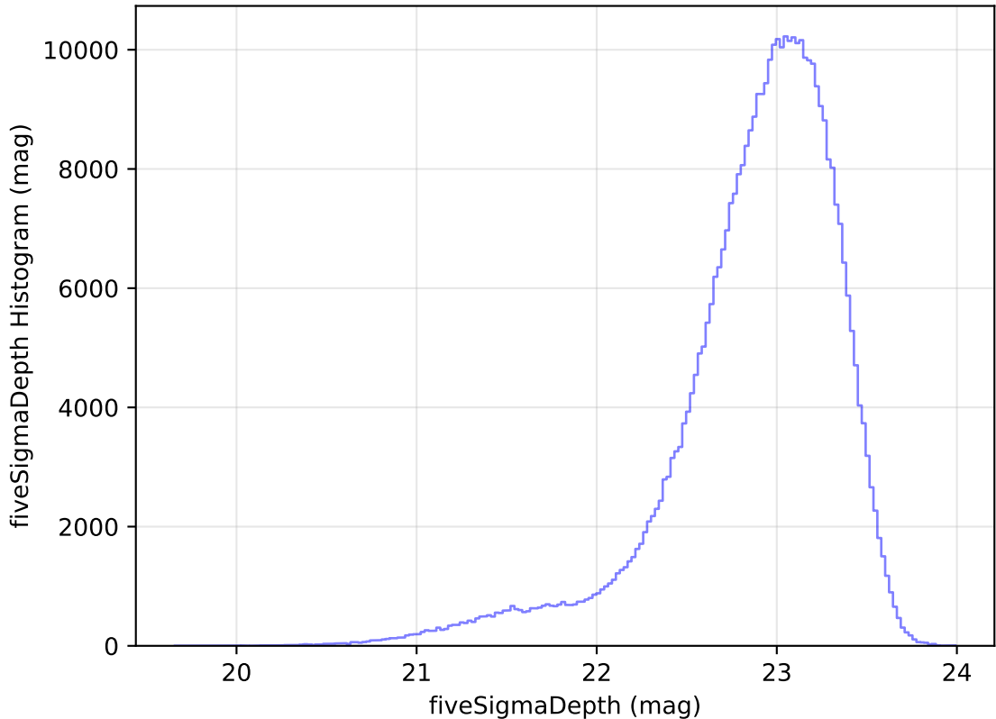
ddf_acor_sf15_lsf40_lsr10_v3.4_10yrs WFD z band: fiveSigmaDepth Histogram
