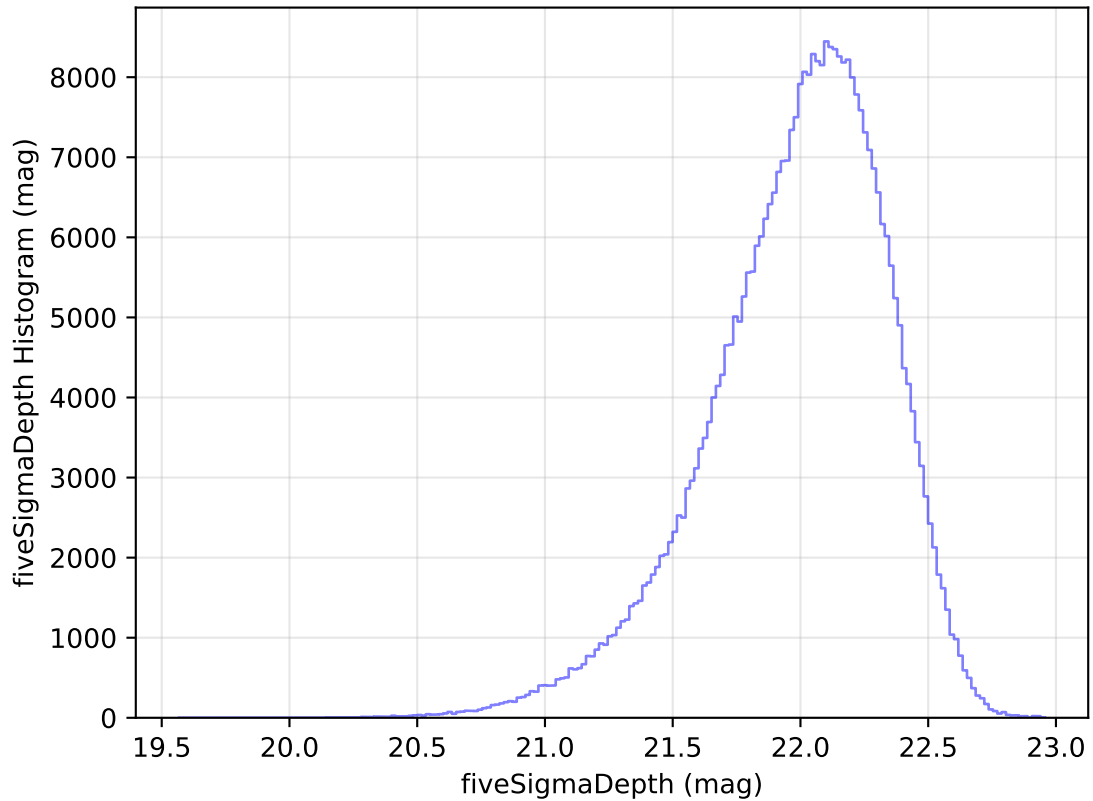
ddf_acor_sf15_lsf40_lsr10_v3.4_10yrs WFD y band: fiveSigmaDepth Histogram
