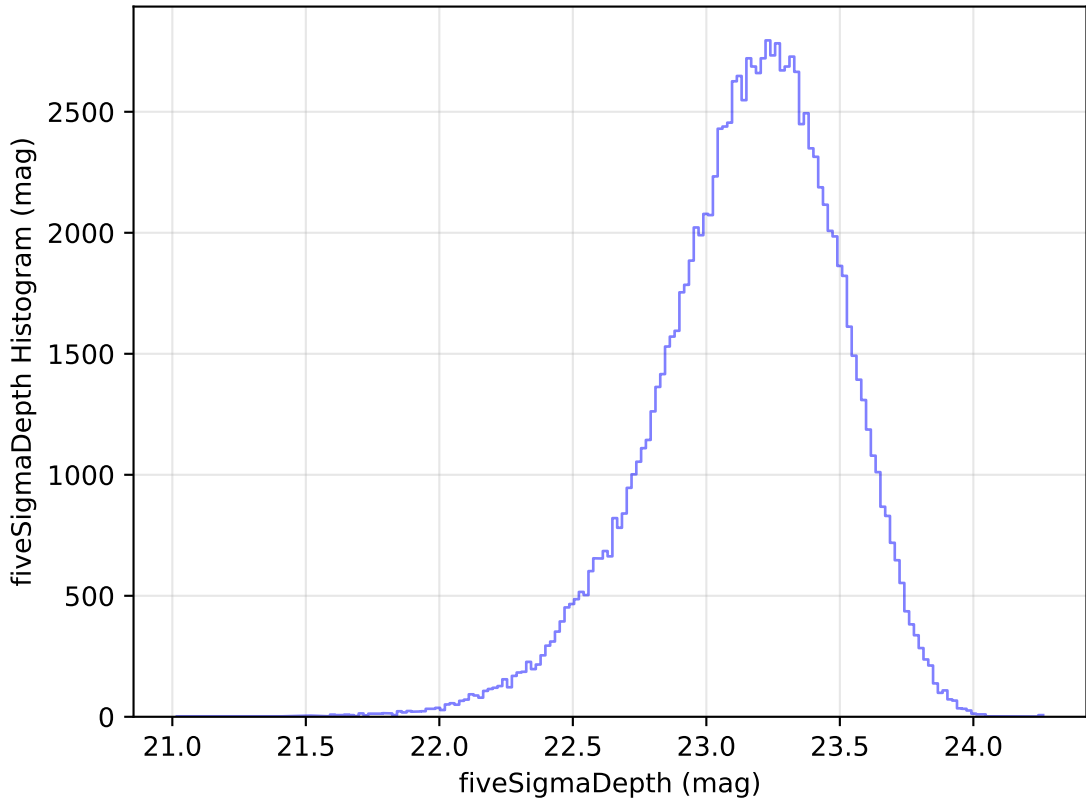
ddf_acor_sf15_lsf40_lsr10_v3.4_10yrs WFD u band: fiveSigmaDepth Histogram
