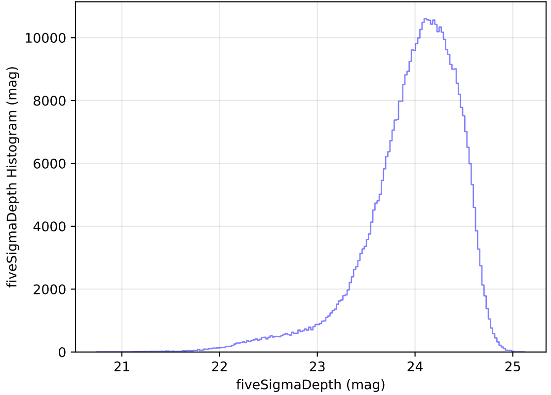
ddf_acor_sf15_lsf40_lsr10_v3.4_10yrs WFD r band: fiveSigmaDepth Histogram
