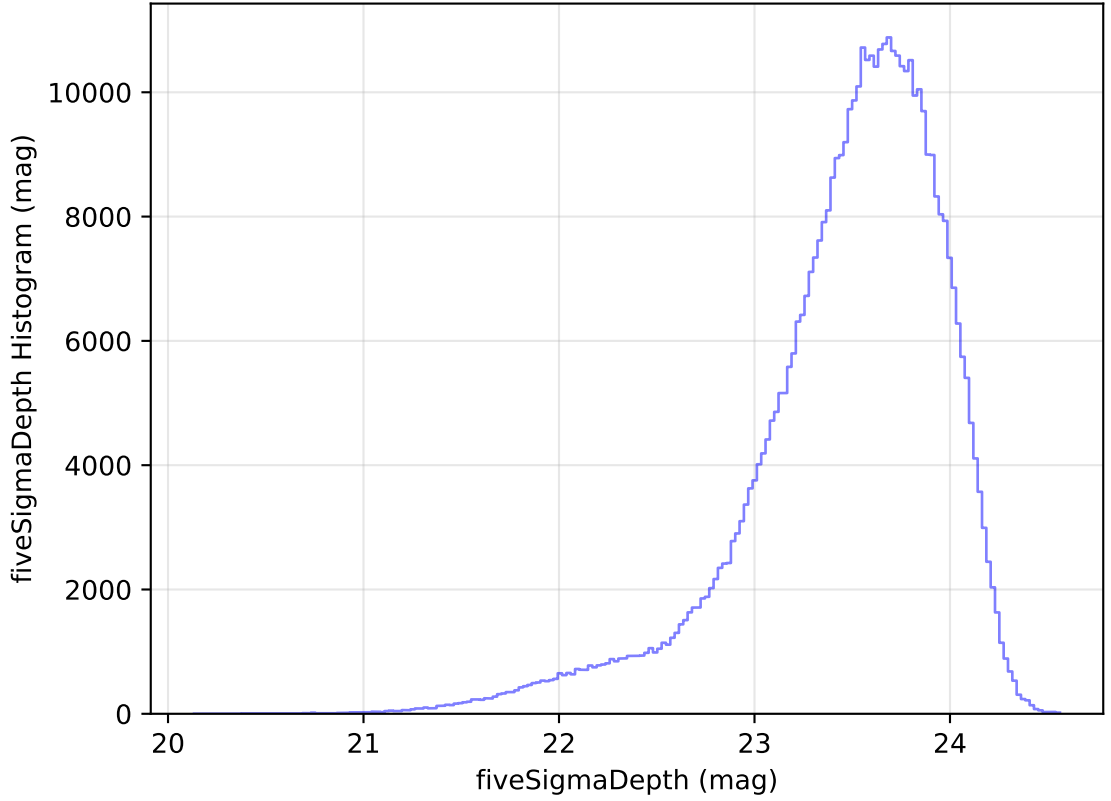
ddf_acor_sf15_lsf40_lsr10_v3.4_10yrs WFD i band: fiveSigmaDepth Histogram
