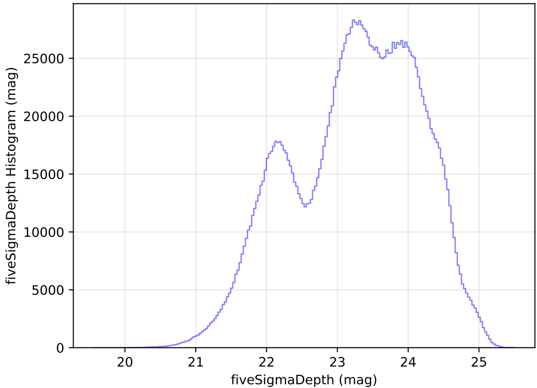
ddf_acor_sf15_lsf40_lsr10_v3.4_10yrs WFD all bands: fiveSigmaDepth Histogram
