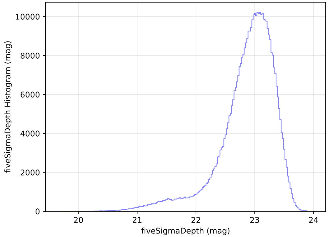
ddf_acor_sf15_lsf40_lsr10_v3.4_10yrs All sky z band: fiveSigmaDepth Histogram
